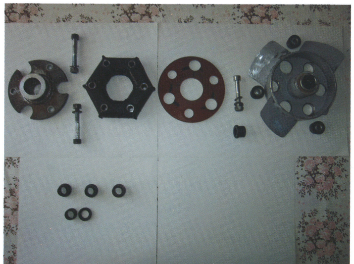
MUTC disassembled trolley bus hardy clutch system
