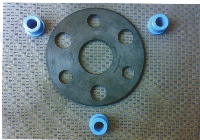
Replacement of clutch Tecamid parts with ThorPlas-Blue
