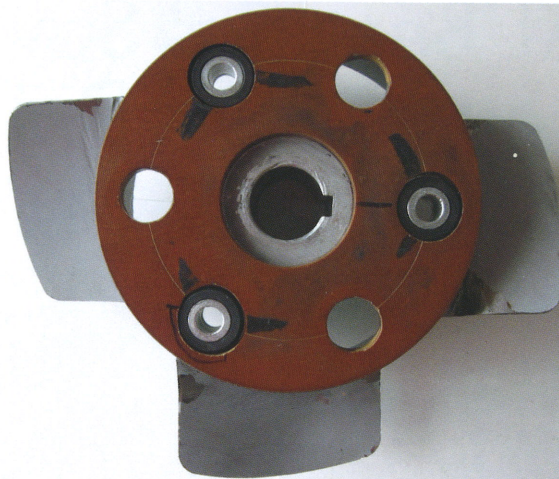
Replacement of clutch Pentinax part with Thordon XL
